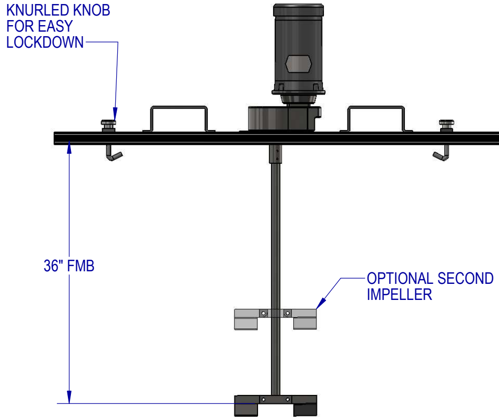
BRIDGE MOUNT TOTE MIXERS MOUNT TO CAGE STYLE TOTES UP TO 52" WIDE
